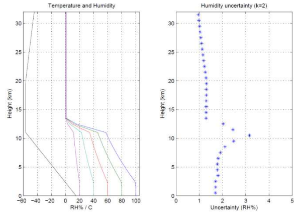
Figure 9: The combined measurement uncertainty of RS41 humidity measurement ( k=2 ). The uncertainty analysis model applied U.S. Standard Atmosphere 1976 temperature profile and a set of humidity profiles (left), and the resulting humidity measurement uncertainty (right).
