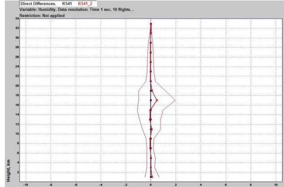
Figure 28: RS41-RS41 humidity reproducibility in tropical daytime atmosphere
