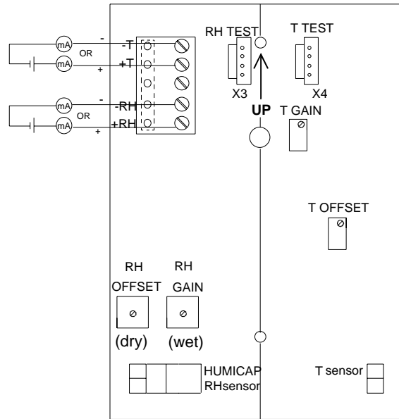
Figure 3.3 Electrical connections
