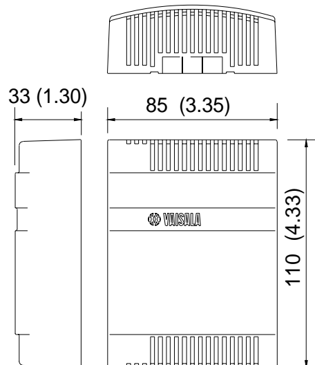
Figure 3.2 Dimensions of the HMW60U/Y (in mm)
