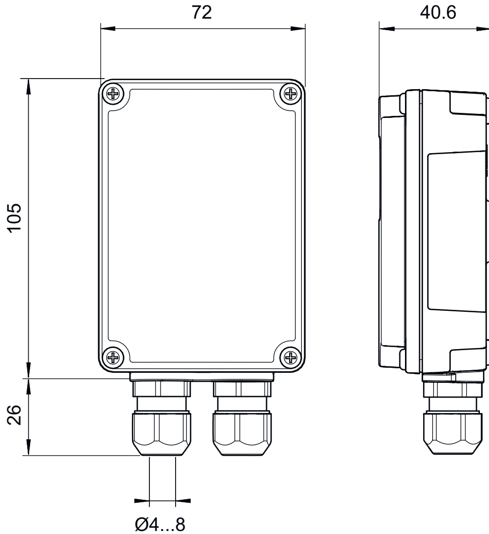
Figure 2 GMP250 Relay Box Dimensions
