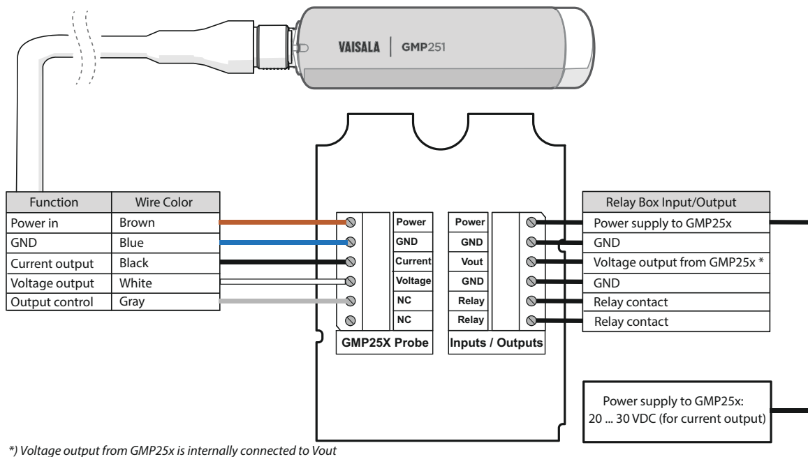
Figure 1 Probe and Relay Box Wiring
