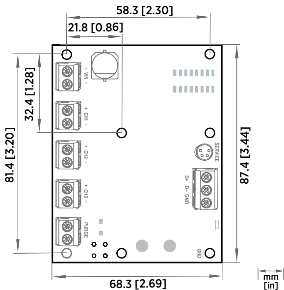
Figure 2 HMM170 component board dimensions
