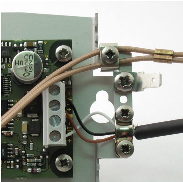
Figure 4 Connecting Cables
