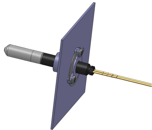
Figure 3 Mounting the Flange Through Wall
