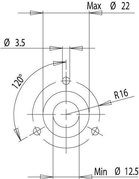
Figure 6 Mounting Hole Dimensions
