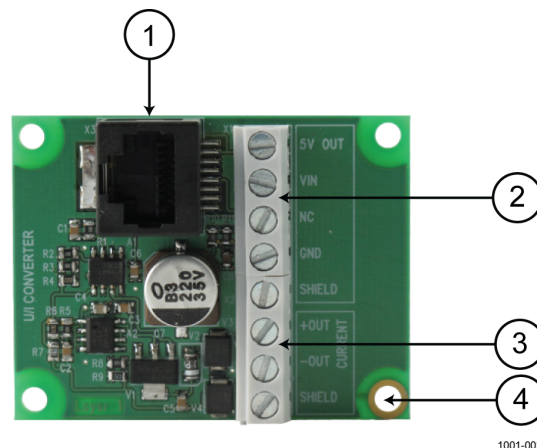
Figure 1 Loop Power Converter
