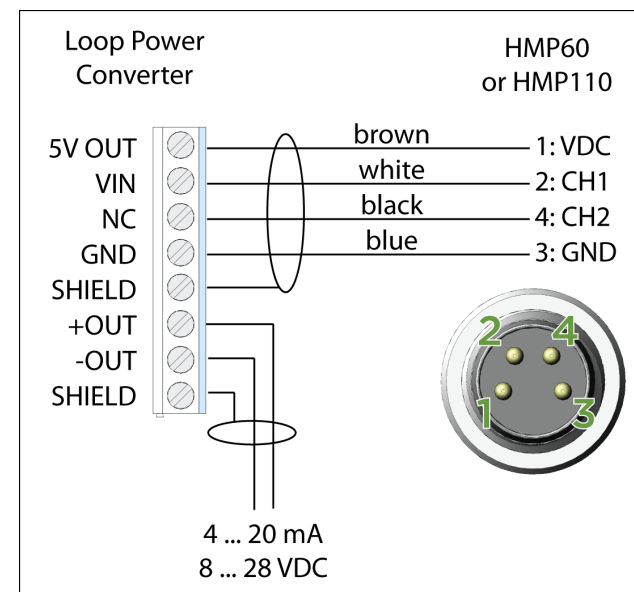
Figure 2 Wiring with HMP60 or HMP110
