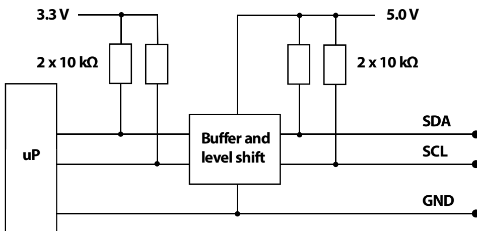
Figure 1 Hardware Schematic
