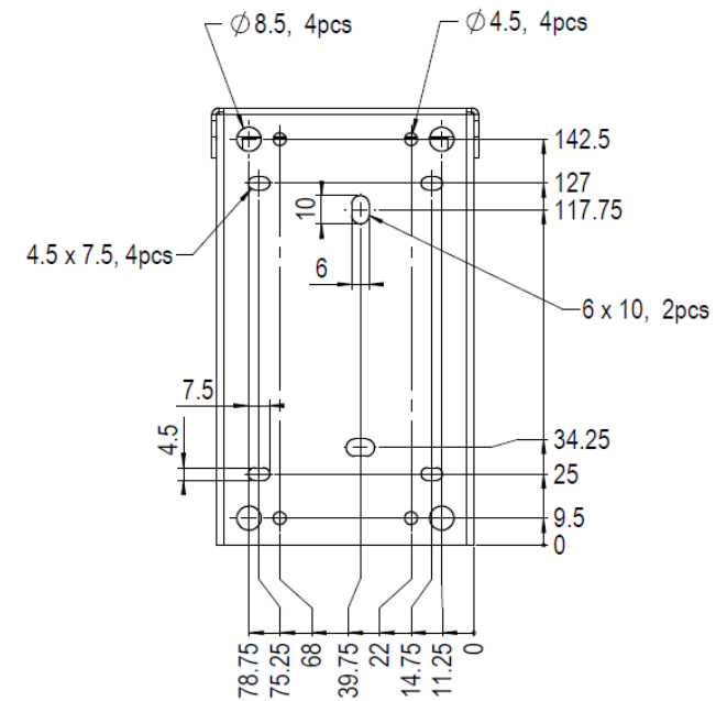
Figure 3 Rain Shield Dimensions (Back)
