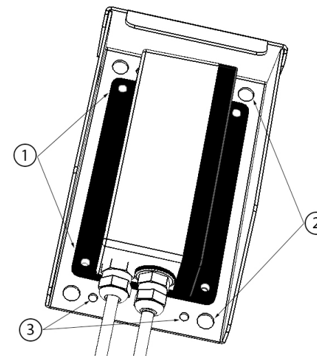
Figure 2 Rain Shield Mounting Options
