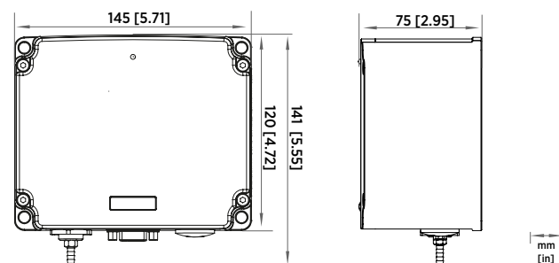
PTB330AWS dimensions
